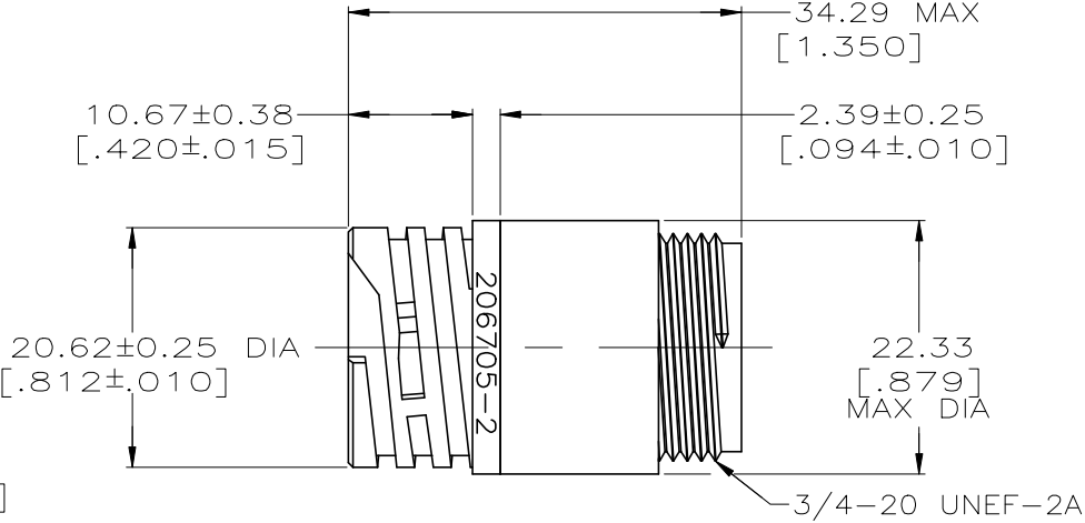
DETAIL A
