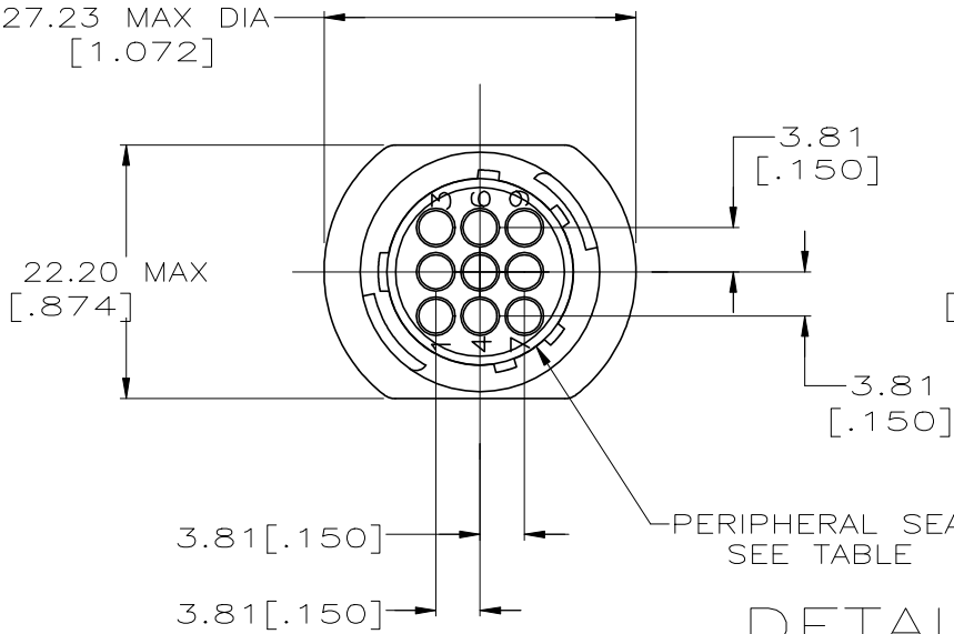
DETAIL B
