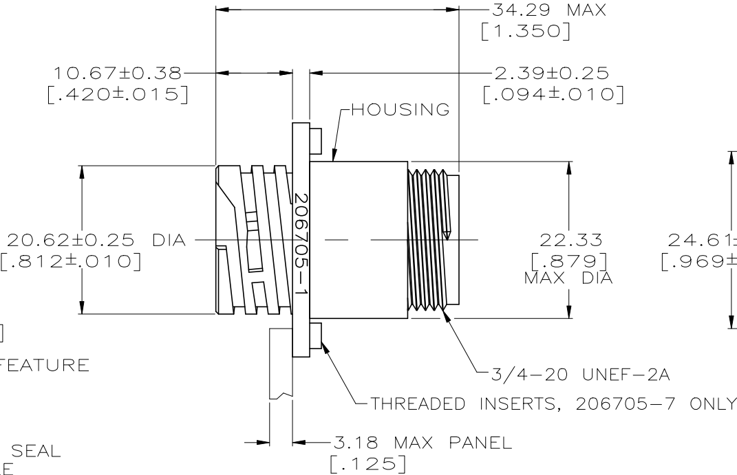
DETAIL A
