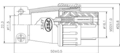
PLS-20◆-PF X-R
