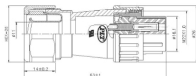
PLS-20◆-GPF3 X-R
