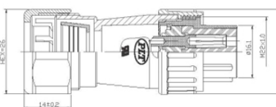
PLS-20◆-WGP3 X-R
