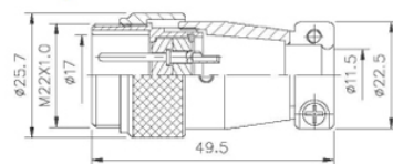
PLS-20◆-ADM-R
