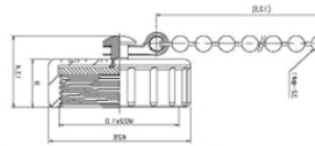
PLS-20C-RCaC-R
