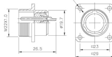
PLS-20◆-RM-R
